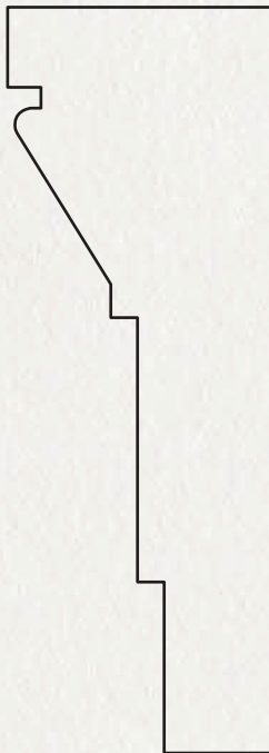
KB407 1-1/4" x 3-1/2"
