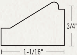
KB246 3/4" x 1-1/16"
