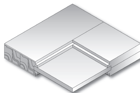
Bravo Flat Panel Square Sticking
