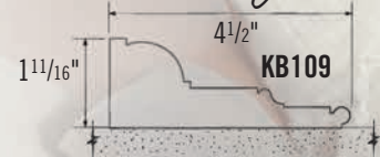
Casing
