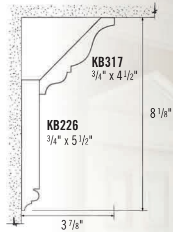
Crown/Cornice
