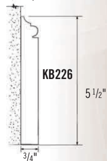
Base
