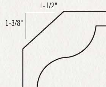
KB319 3/4" x 2" (Supporting Bed Mould)
