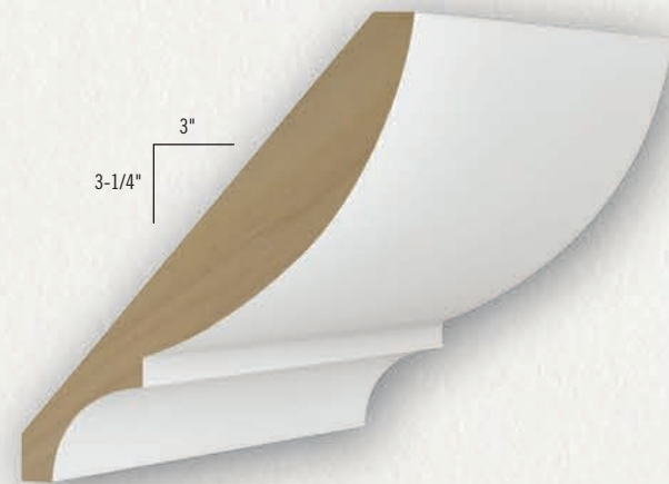
KB313 Crown
