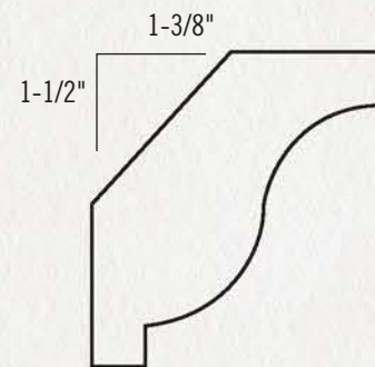
KB319 3/4" x 2" (Terminating Crown)
