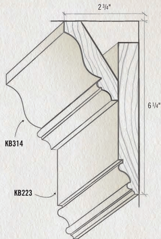
Federal Crown Cornice
