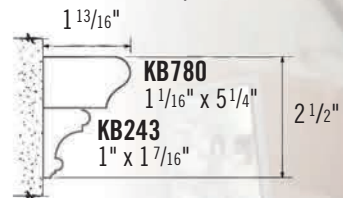
Chair Rail
