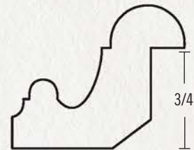
KB881 3/4" x 1-1/2"
