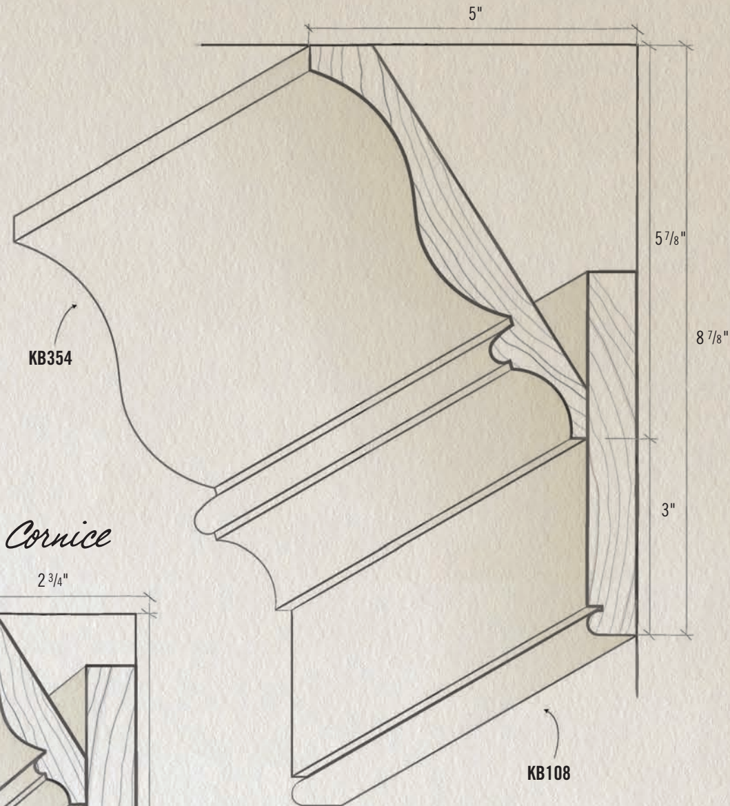
Traditional Revival Cornice
