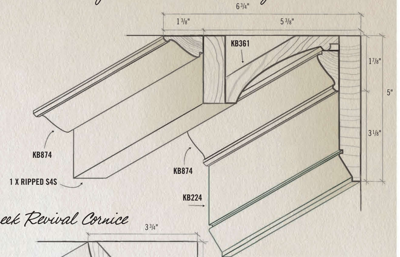
Greek Revival Plaster Style Cornice
