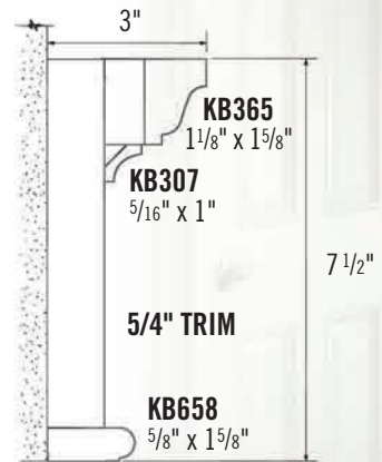
Window/Door Header
