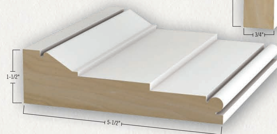
KB117 Casing
