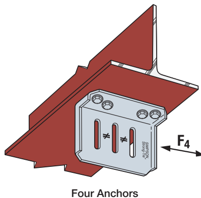
SCW5.5 Anchor Layout
