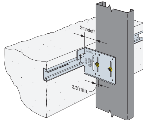
DSSCB Standoff Distance with Concrete Insert and Minimum Fastener Edge Distance for Slide-Clip Application
