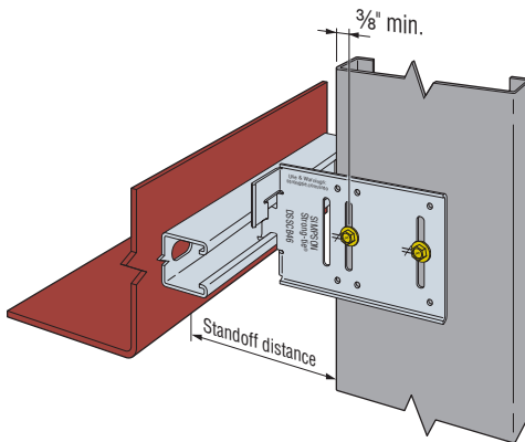
DSSCB Standoff Distance with 1 1/8" Strut (7/8" Strut Similar) and Minimum Fastener Edge Distance for Slide-Clip Application
