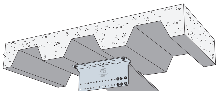
Kickers to Underside of Deck
