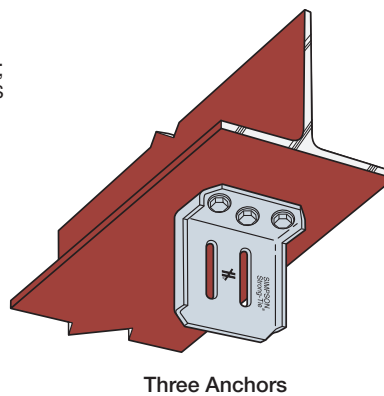
SCW3.25 Anchor Layout
