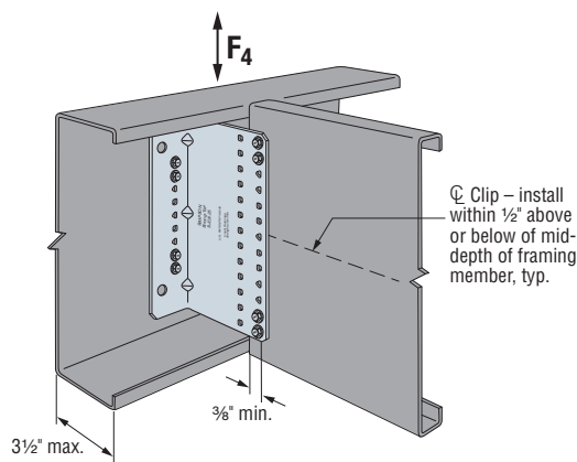
SJC Installation with Carried Member Fasteners in Min. Pattern (fill circle holes min. quantity, circle and triangle holes max. quantity)
