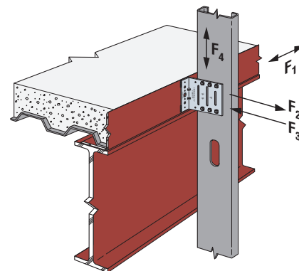
Typical SCS Fixed-Clip Installation
