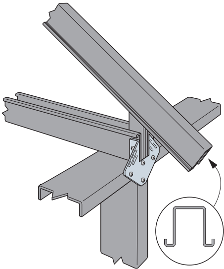
Typical S/H1A Installation
