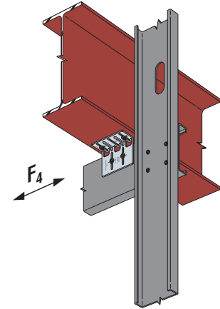
Typical HWDC Installation with Stud Strut
