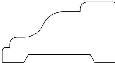
RPVC5287 Rake Moulding 1-1/16" x 2"
