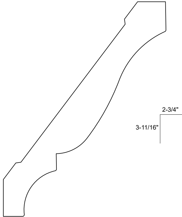
RPVC5047 4-5/8" Crown 5/8" x 4-5/8"
