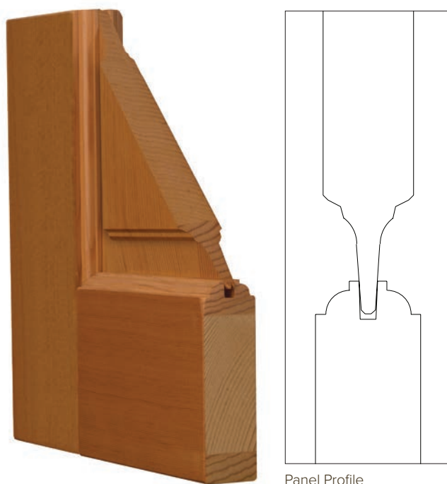
Panel Profile
