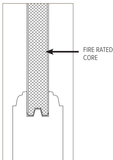
Panel Profile
