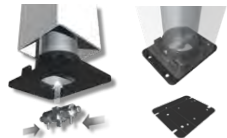
Wind Uplift Base Kit*
