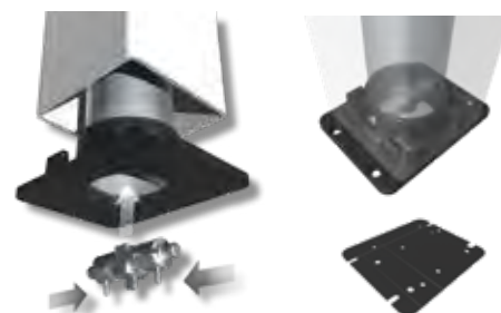
Wind Uplift Base Kit*
