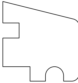
PVC5311 Sill Nosing 1-1/2" x 1-1/4"
