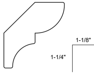
PVC5075 Bed Mould 1/2" x 1-3/4"
