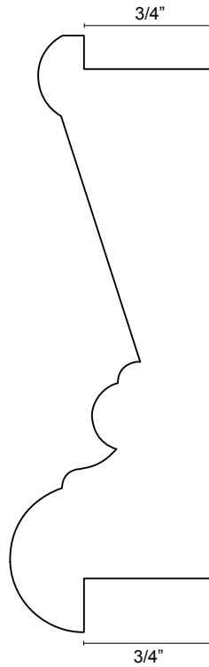
PLP312MDF 1-3/16" x 3-1/2"
