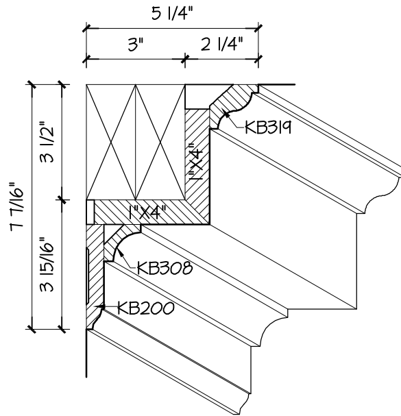
WALL BEAM
