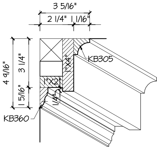
WALL BEAM
