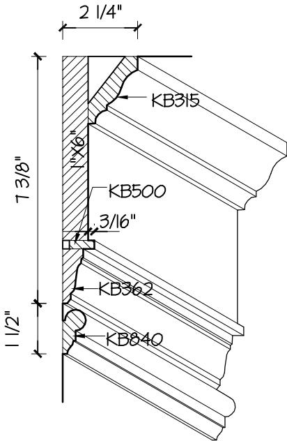
WALL BEAM
