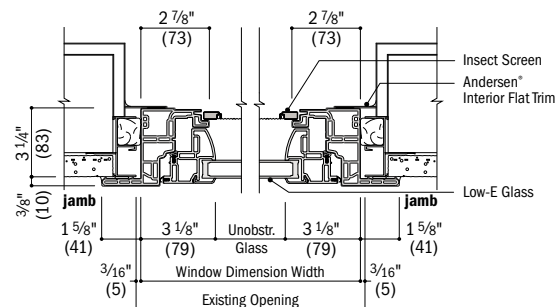
Horizontal Section Existing Aluminum Frame Window Opening
