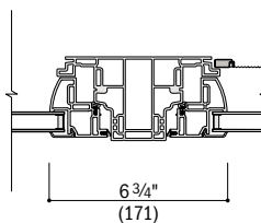
Horizontal Section Picture With Flanking Casement
