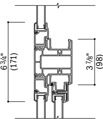
Vertical Section Picture Over Gliding
