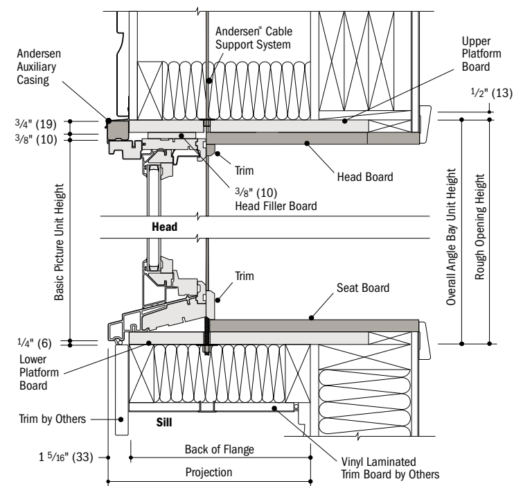
Vertical Section
