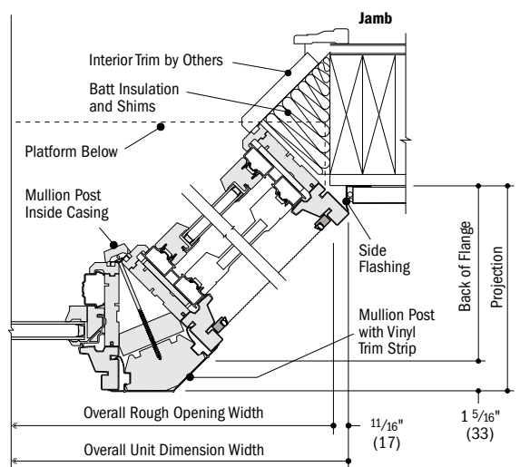
Horizontal Section
