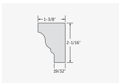
Rams Crown #5158R16
