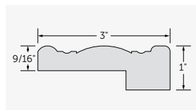
Wainscot Cap/Base #2566R8
