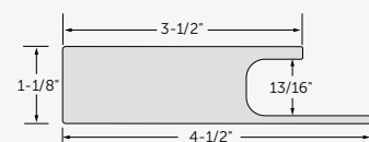
J-Channel Casing #7968R16, #7968R18
