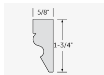
Band Moulding #5168R16
