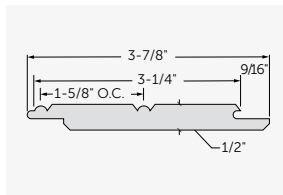
4" KLEERLok® Beaded Board
