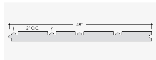
KLEERBeed® Beaded Sheets
