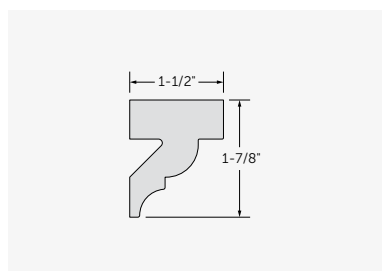
Deco Crown #7712R16
