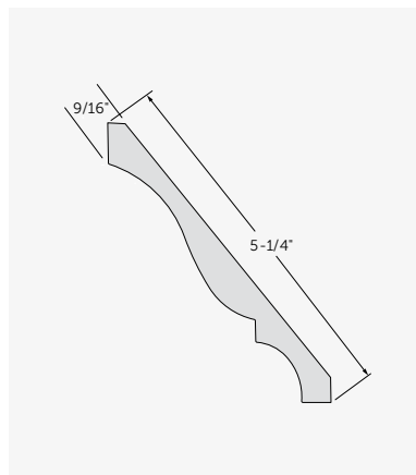
5-1/4" Crown Moulding #5045R16
