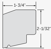
Historic Sill Nose #7650R16
