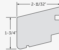
Large Historic Sill Nose #7435C16
