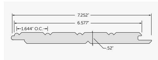
8" KLEERLok® Beaded Board
