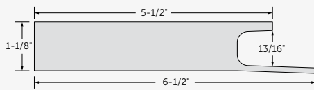
J-Channel Casing #7651R18
