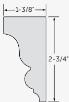
Imperial Rake Moulding #7962R16
