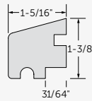
Sill Nose #5311R16
