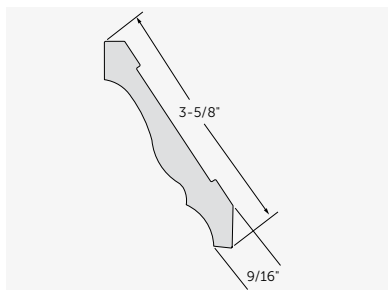
3-5/8" Crown Moulding #5049R16
