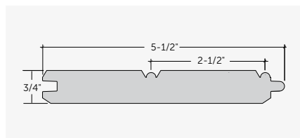
Edge and Center Bead Board
