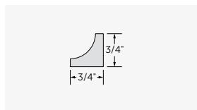
Cove/Scotia #5245R16
