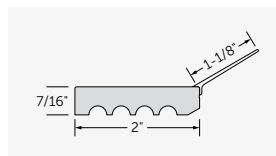
Weather Stop #7951R16
