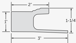
J-Channel Brick Mould #5657R17
