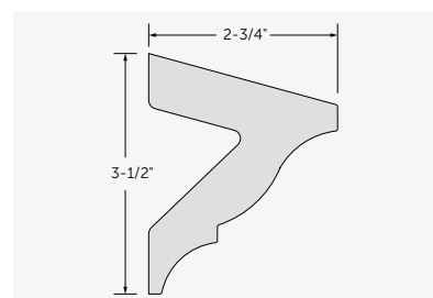
One Piece Crown #7960R12
