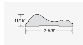
Chair Rail #5390R8
