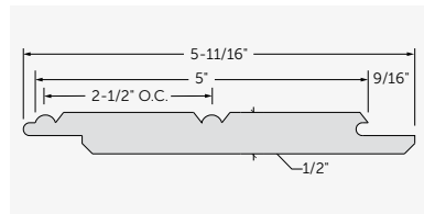
6" KLEERLok® Beaded Board
