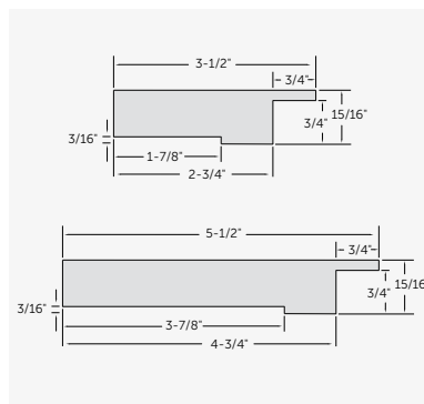
Kleer Konceal® Trimboard with Nailing Flange Cutout
