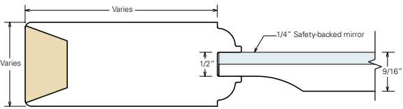
Sample cross section (one-sided mirror door)
