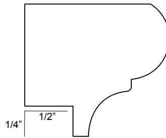
KB810 1-3/8" x 1-1/2"
