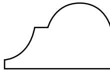
KB392 Nose and Cove 1 1/16" x 1-1/8"
