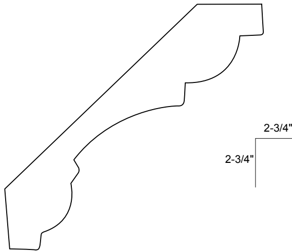
KB340 9/16" x 3-5/8"
