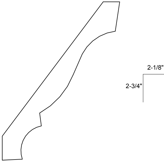
KB320 9/16" x 3-1/2"
