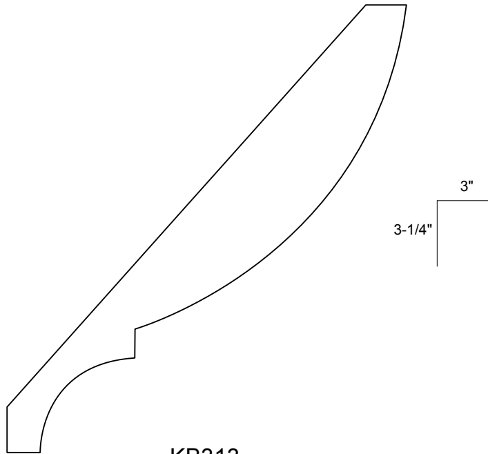
KB313 3/4" x 4-1/2"
