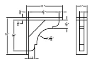
Optional Flower Box - Decorative Bracket #3
