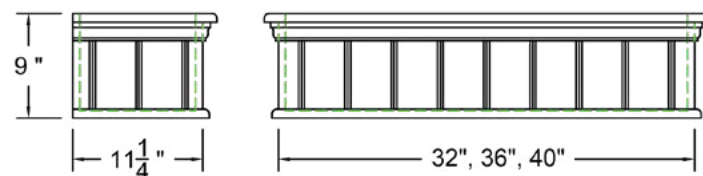
V-Grooved Panel Window Flower Box
