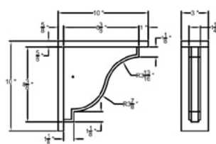
Optional Flower Box - Decorative Bracket #2 Chamfered
