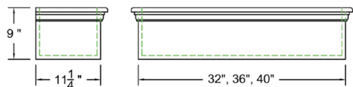
Flat Panel Window Flower Box
