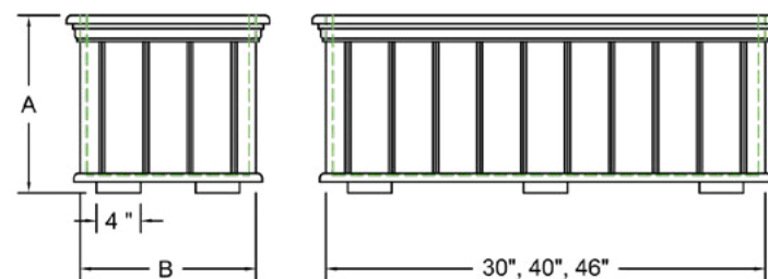
V-Grooved Panel Planter Box
