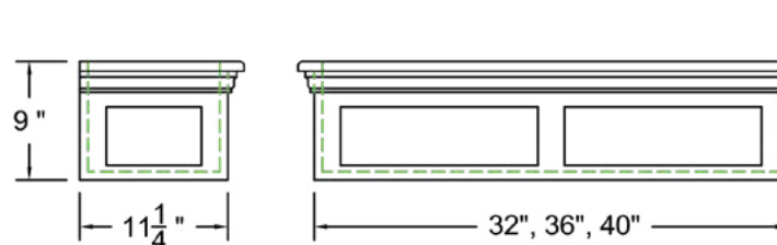
Recessed Window Flower Box
