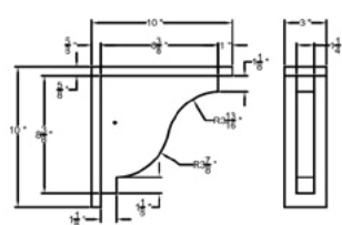
Optional Flower Box - Decorative Bracket #1
