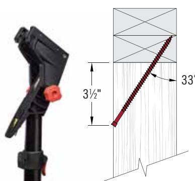
Stud-to-Plate
