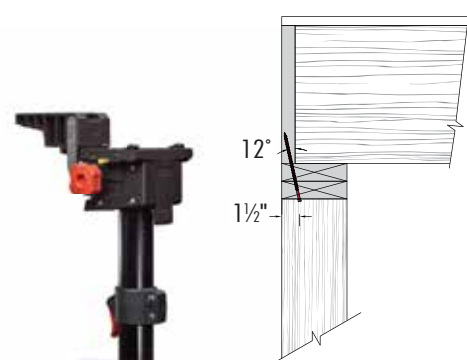
Plate-to-Rim
