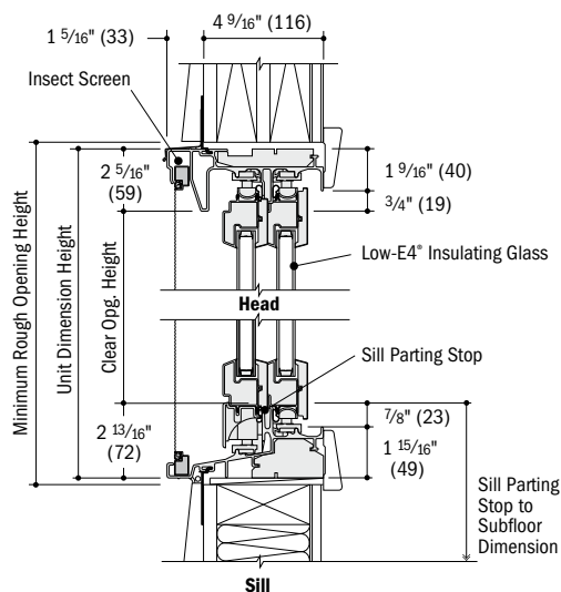
Vertical Section
