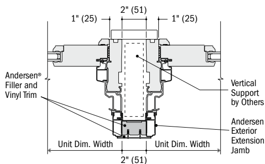
Horizontal Section
