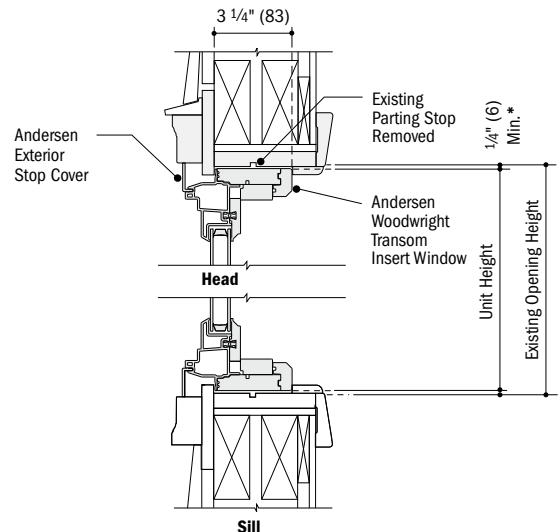
Vertical Section
