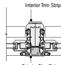
Horizontal Section
