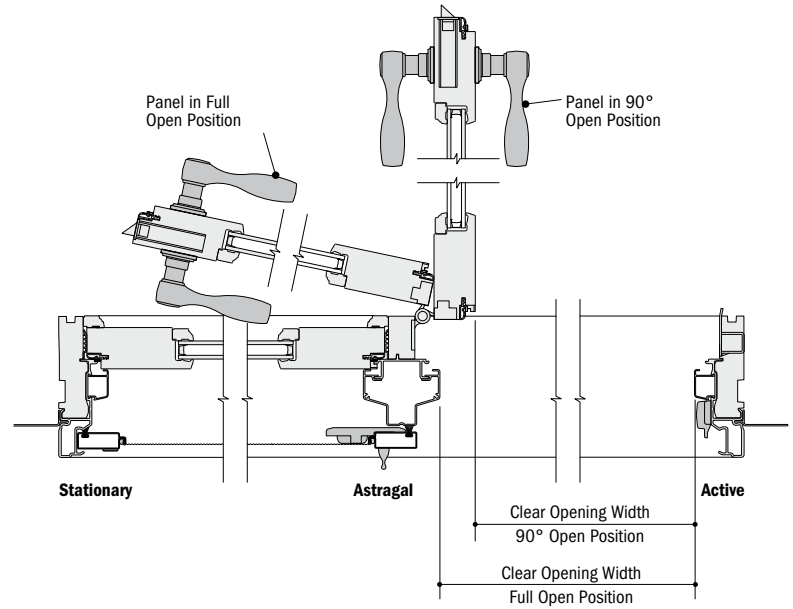
Horizontal Section Two-Panel, Stationary-Active (open)
