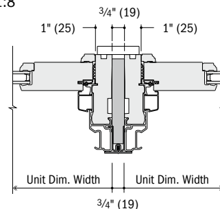
Horizontal Section
