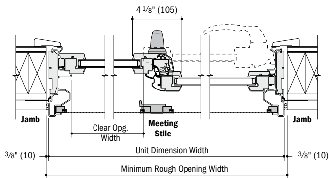
Horizontal Section
