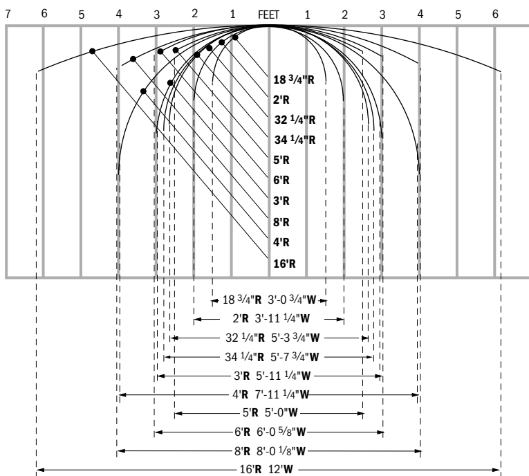
Standard Radii & Maximum Unit Width for Custom Arch Windows
