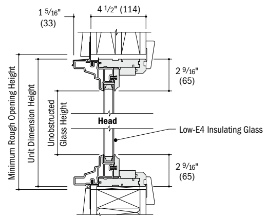
Vertical Section
