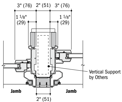
Horizontal Section Gliding and Gliding
