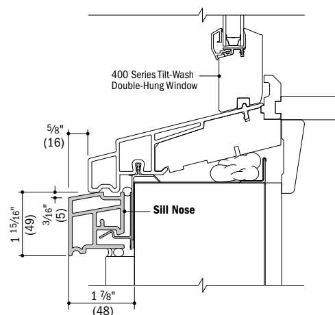
Vertical Section
