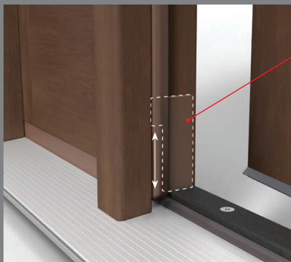
Jamb Assembly with 7-Shape Corner Seal Pad
