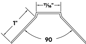
Chamfer Bead® & Archway, Medium
