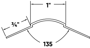
Bullnose Splayed Corner Bead, 3/4" Large
