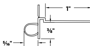
Super Seal Tear Away® L Bead
