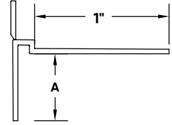
Tear Away® L Bead
