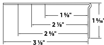
Super Seal Tear Away® L Bead
