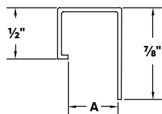
Shadow Line J Bead
