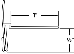
Rigid Jumbo Low Profile Corner Bead & Archway
