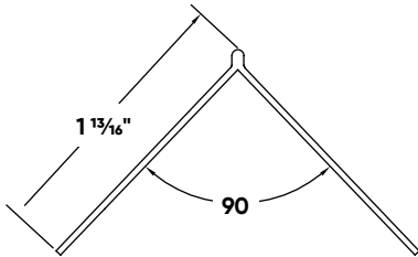
Rigid Low Profile Corner Bead & Archway
