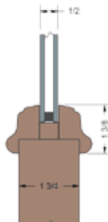
Raised Molding 1/2" I.G.
