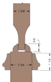
Recessed Molding WB31 Bolection Standard Panel
