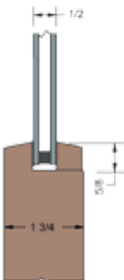
Tapered Mission Molding 1/2" I.G.
