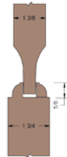
Recessed Molding Standard Panel
