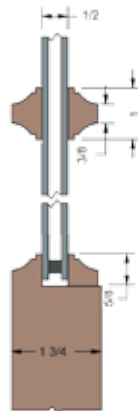
Recessed Molding Style B & 1" SDL Bar
