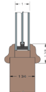
Raised Molding 1" I.G.
