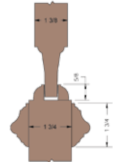
Recessed Molding W/ WB21 Bolection Classical Panel
