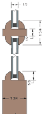
Recessed Molding & 1 3/4" TDL Bar
