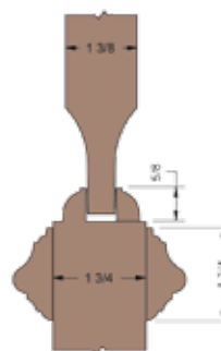
Recessed Molding WB21 Bolection Standard Panel
