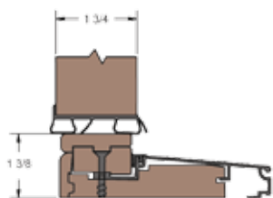
Impact Inswing Sill
