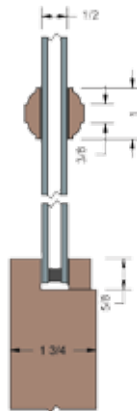
Mission Molding & 1" SDL Bar
