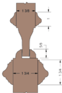
Recessed Molding WB21 Bolection and WB11 Bolection on Ogee Panel
