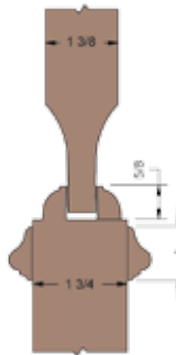
Recessed Molding WB11 Bolection Standard Panel
