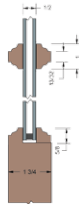
Recessed Molding Style C & 1" SDL Bar
