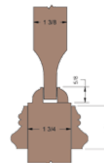
Recessed Molding WB41 Bolection Standard Panel
