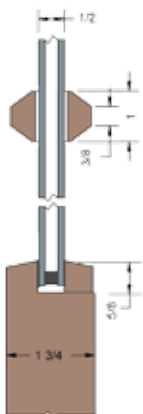
Tapered Mission Molding & 1" SDL Bar
