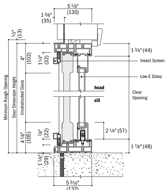
Vertical Section
