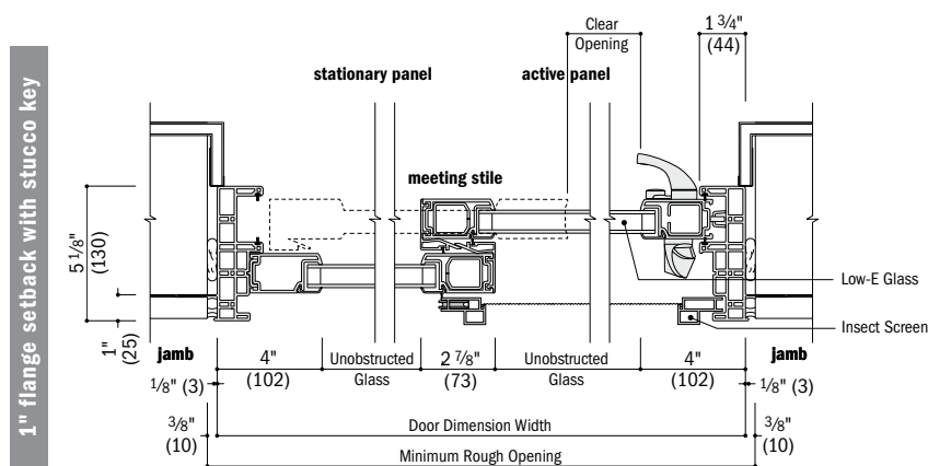
Horizontal Section
