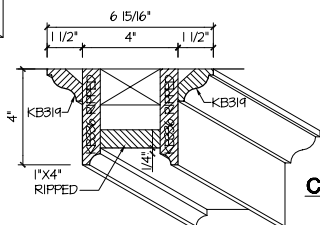
WALL BEAM
