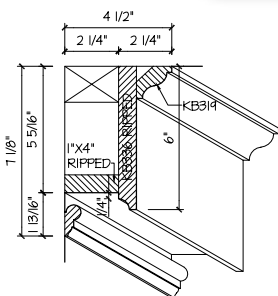
WALL BEAM
