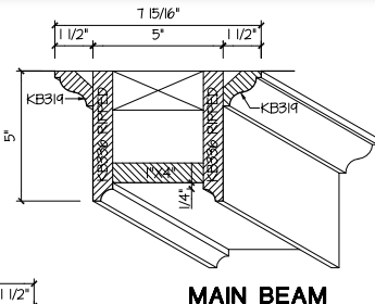
MAIN BEAM
